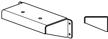
Arm Mount Brkt 1061-940910
